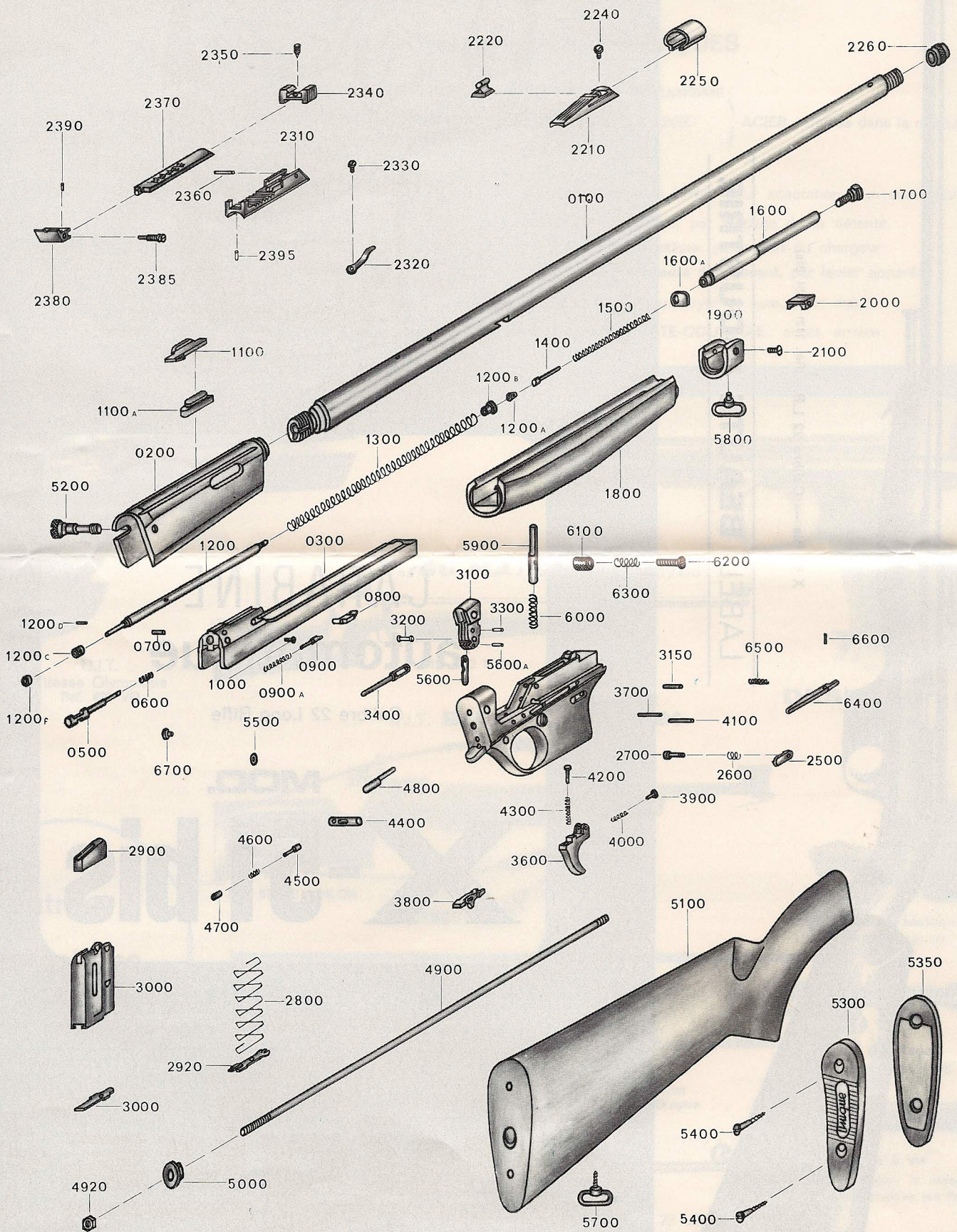
PERSPECTIVE ECLATEE DES PIECES CONSTITUTIVES
